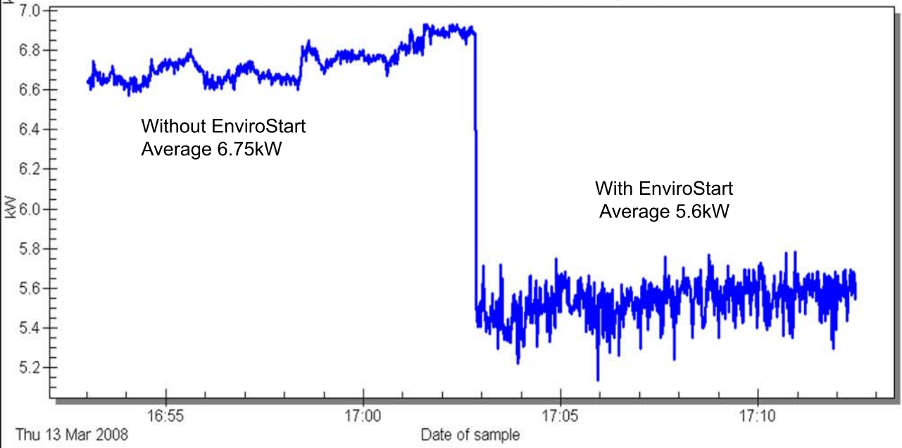
Denco, Hereford, UK 7.5kW AC Compressor
